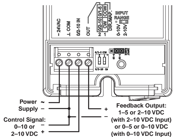
Illustration 5—MEP-4xx2 Proportional Wiring
